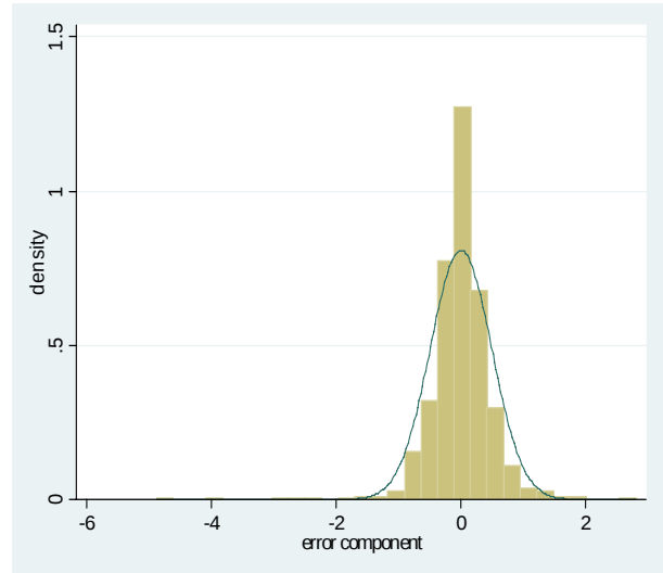
Figure 1: Residual Analysis
